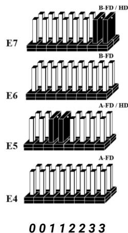
Figure 4 – DMA Selection Headers E4 – E7
