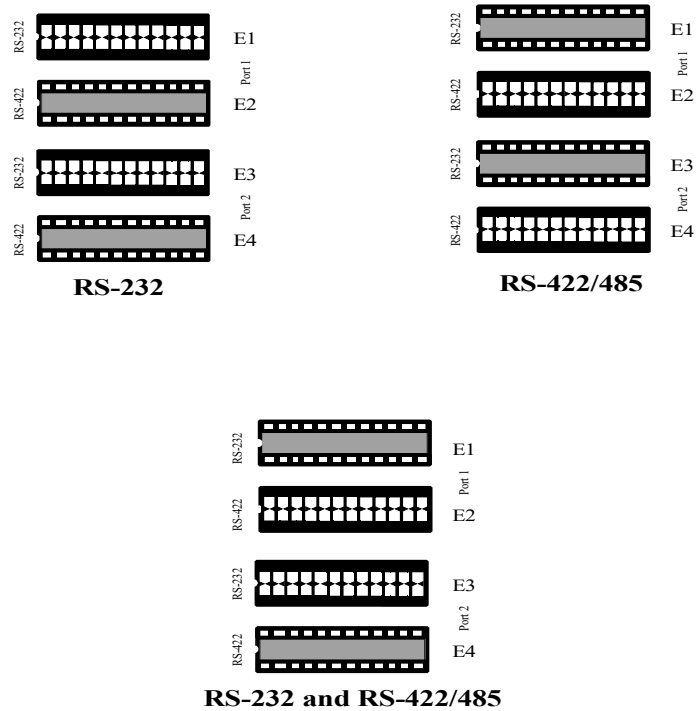
Figure 7 - Headers E1 - E4, Electrical Interface Selection
