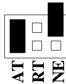
Figure 2 - Headers J1B – J4B, RS-485 'Auto' Enabled, with 'No Echo'
