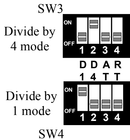
Figure 7 - Clocking Modes
