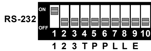
Figure 1- RS-232
